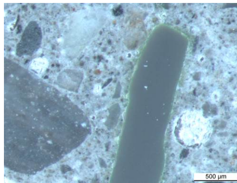
Polymer fiber (A2)
