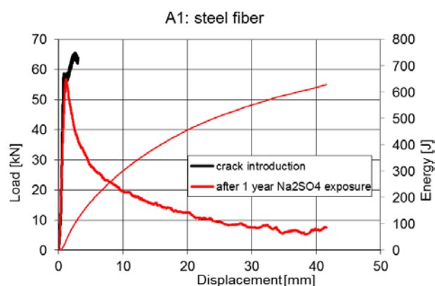
Figure 4 Load displacement curve of steel fiber 1 (A1) after 1 year of exposure to sulfate-solution (4g/l Na 2 SO 4 ).
