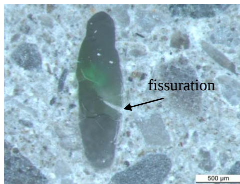
Polymer fiber (A5)
