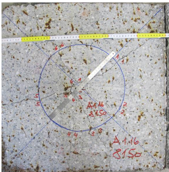
Figure 7 Photo of steel fiber reinforced square panel (A1) after 1 year of exposure to Salt (NaCl-solution: 3%).
