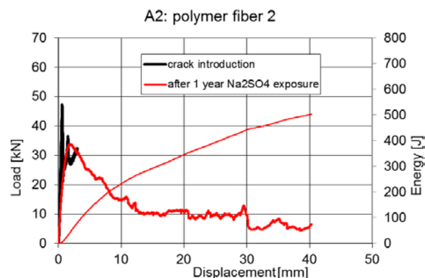
Figure 5 Load displacement curve of polymer fiber 2 (A2) after 1 year of exposure to sulfate-solution (4g/l Na 2 SO 4 ).
