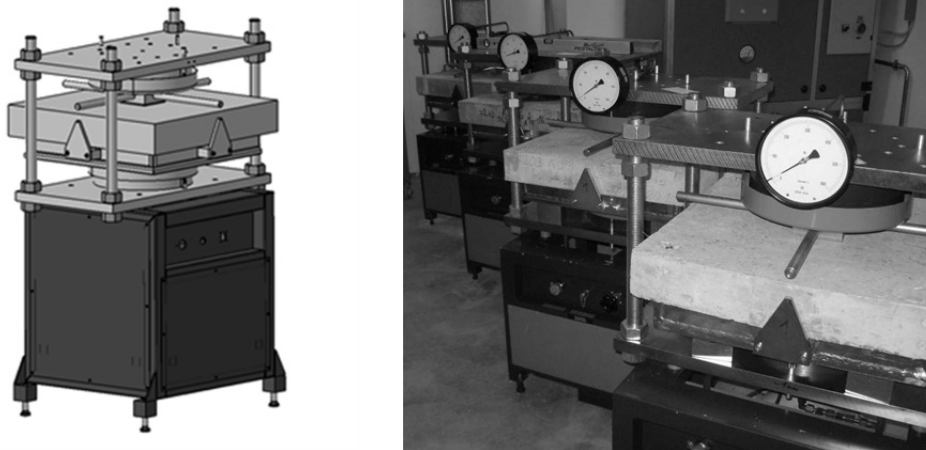
Figure 2 Test arrangement of creep tests on square panels under constant load
